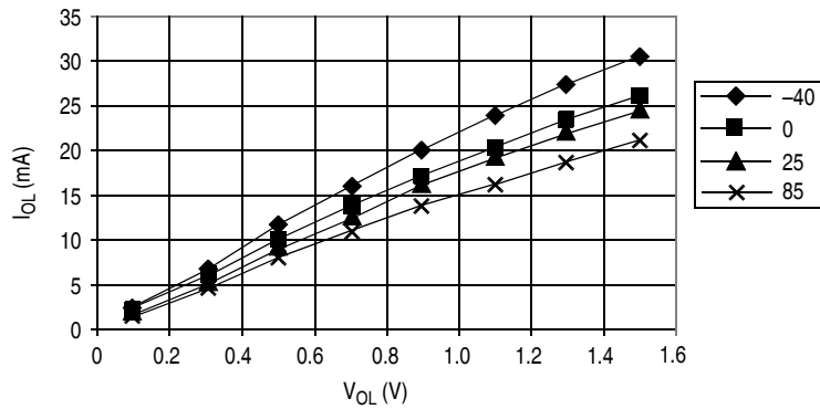
Figure 20-9. Typical Low-Side Driver Characteristics – Port PTA7–PTA0 ( V_{DD} = 5.5 Vdc)
