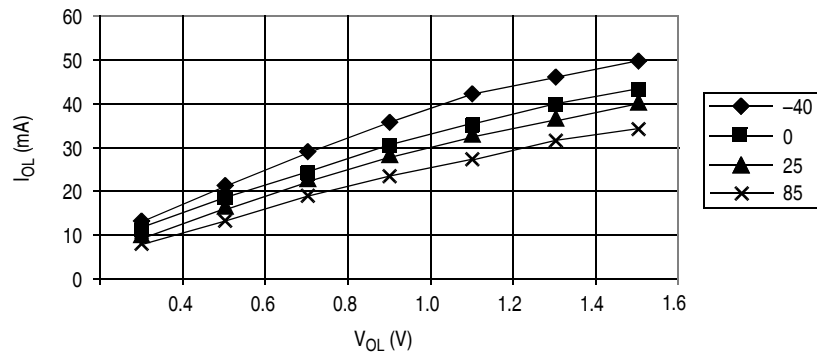
Figure 20-11. Typical Low-Side Driver Characteristics – Port PTC4–PTC0 ( V_{DD} = 4.5 Vdc)
