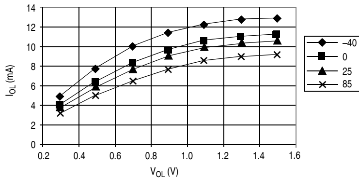
Figure 20-10. Typical Low-Side Driver Characteristics – Port PTA7–PTA0 ( V_{DD} = 2.7 Vdc)
